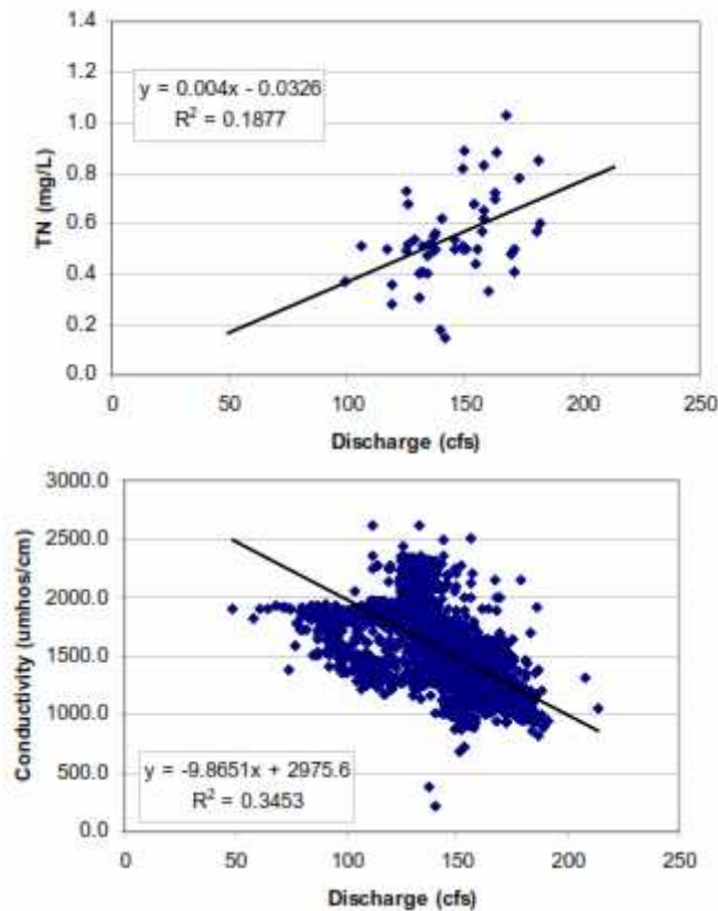
Figure 3.3 Relationships of total nitrogen and conductivity to spring discharge (WSI, 2009)
