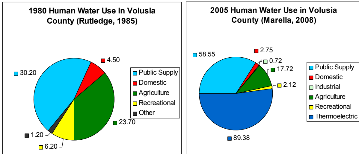
Figure 2.5 Human Water Use in Volusia County in 1980 and 2005 (Rutledge, 1985 and Marella, 2008)
