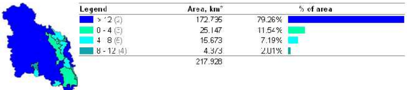
Figure 2.3 Recharge to the Floridan Aquifer in inches per year (SJWMD, 1995)
