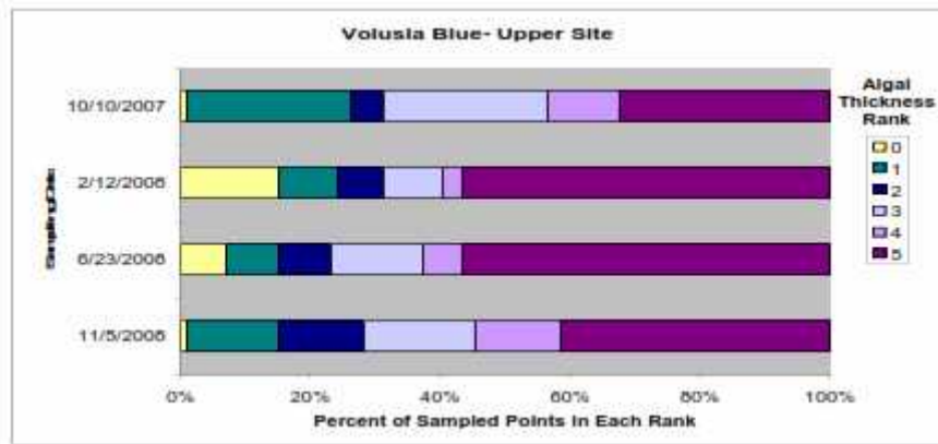
Figure 3.4 Filamentous algae thickness for Upper Blue Spring Run (FDEP, 2009)
