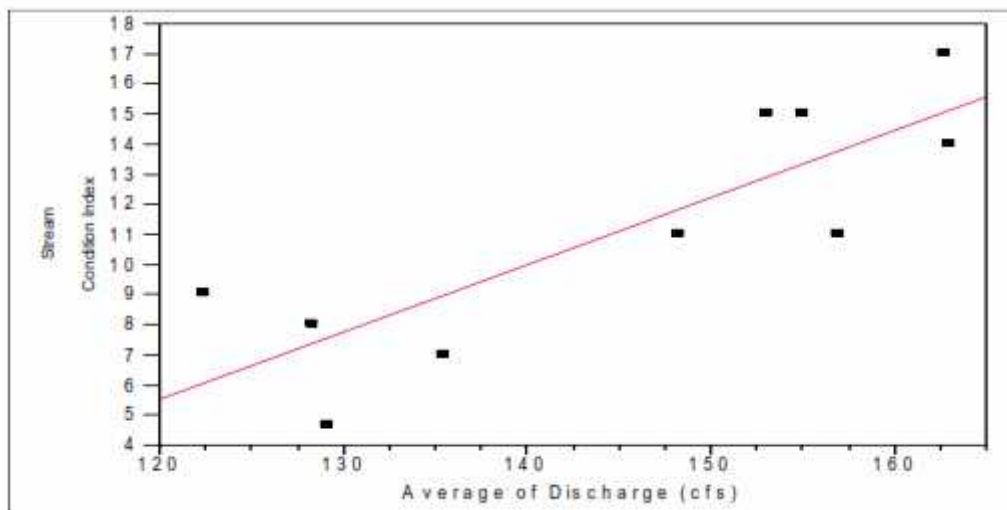
Figure 3.2 Relationship of SCI to average spring discharge from 2000 to 2008 (WSI, 2009)
