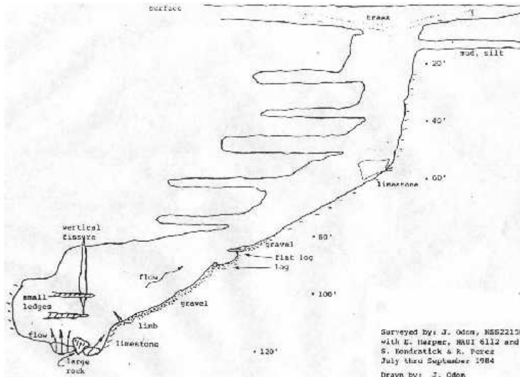
Figure 1.2 Profile of the Blue Spring main vent drawn by J. Odom (WSI, 2009)
