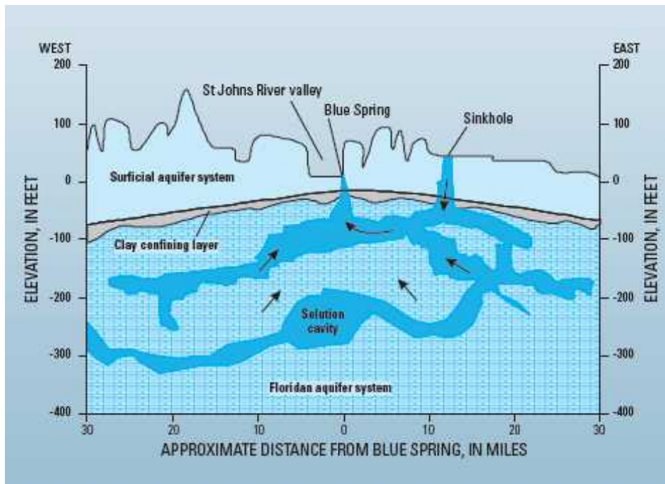
Figure 2.1 Generalized cross-section west to east of Blue Spring by USGS (German, 2008)
