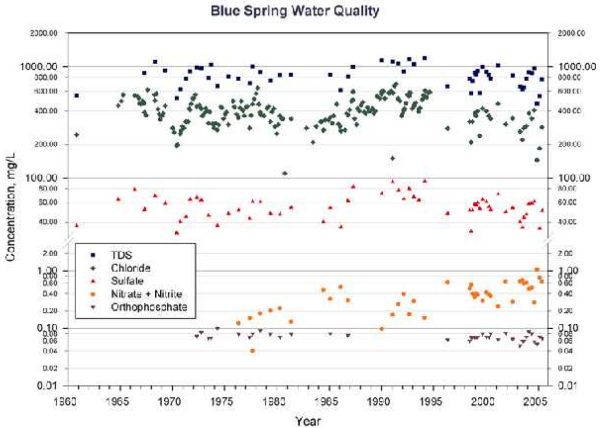
Figure 1.4 Water Quality concentrations from 1960-2005 (SJWMD, 2010)
