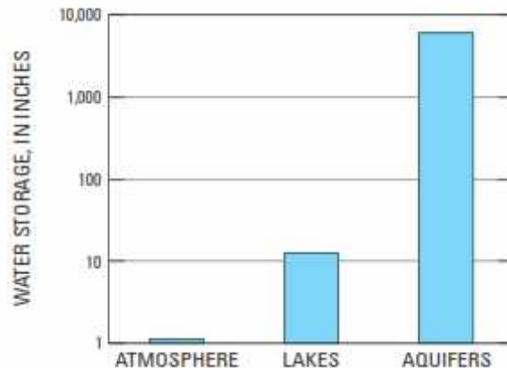
Figure 2.7 Estimated Average Water Storage in Volusia County (German, 2009)
