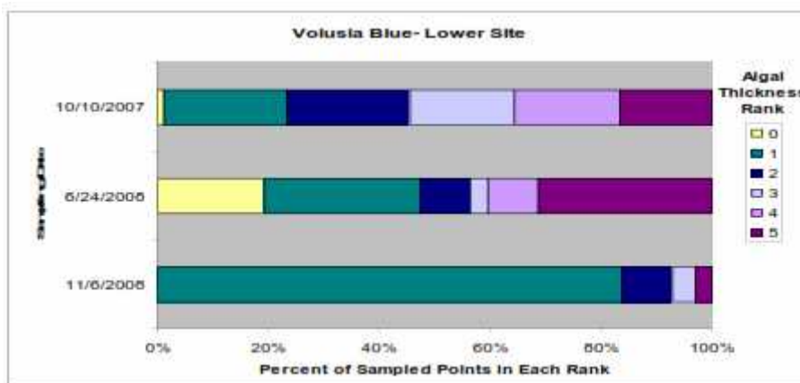
Figure 3.6 Filamentous algae thickness for Lower Blue Spring Run (FDEP, 2009)
