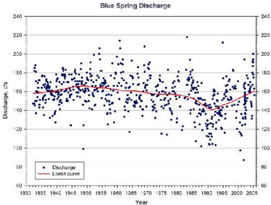
Figure 1.3 Discharge in cubic feet per second from 1932 to 2005 (SJWMD, 2010)
