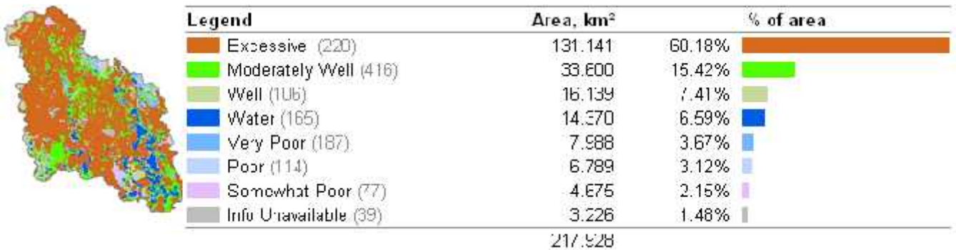
Figure 2.2 Soils Drainage in the Blue Spring Watershed (SJWMD, 2001)
