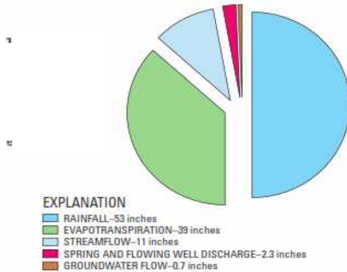
Figure 2.6 Annual Water Budget in Volusia County (German, 2009)
