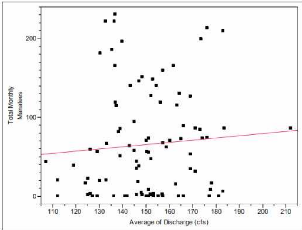
Figure 3.1 Relationship of monthly manatee numbers to average spring discharge from 1983 to 2008 (WSI, 2009)
